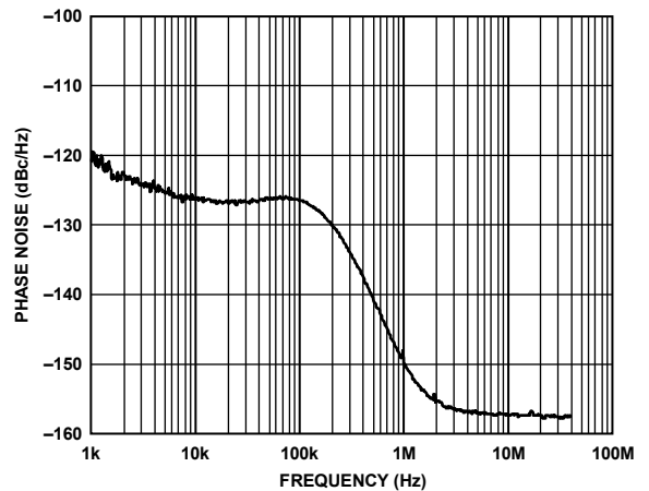
Figure 10. Phase Noise, PLL1, OUT0 LVPECL, 125 MHz, Integer-N Mode ( f_{XTAL} = 25 MHz, N_a = 100 , V_0 = 4 , D_0 = 5 )
