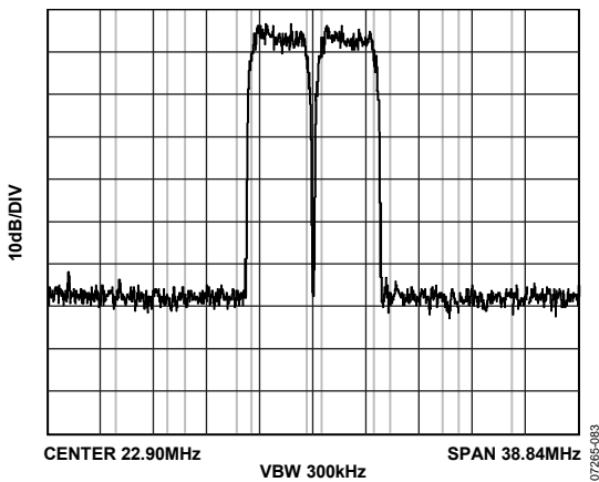
Figure 62. AD9717 ACLR 2-Carrier 1.8 V
