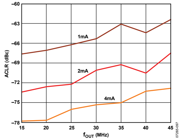
Figure 46. 1 Carrier ACLR First Adjacent Channel at 3.3 V
