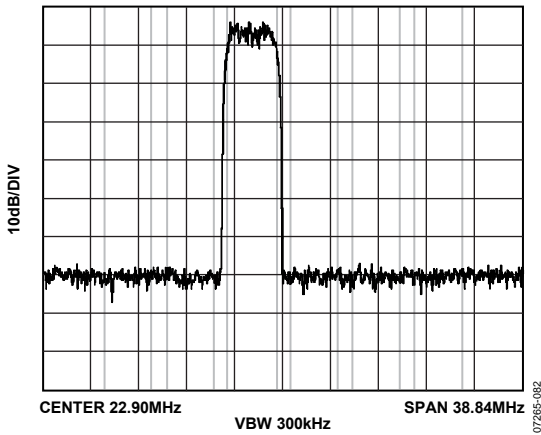
Figure 61. AD9717 ACLR 1-Carrier 3.3 V
