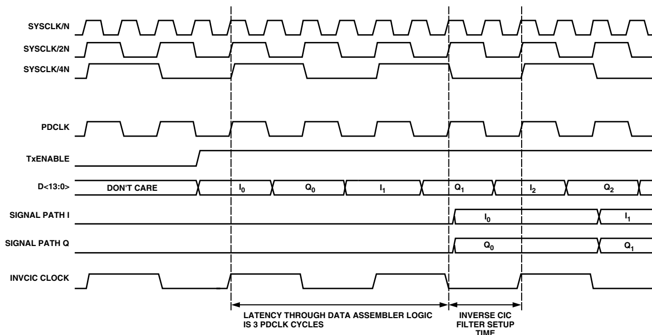
Figure 31. Latency from D\langle 13:0 \rangle to Signal Processing Chain, Four PDCLK Cycles
