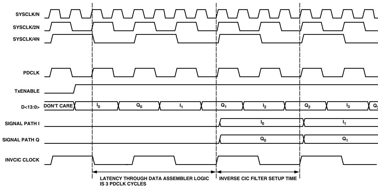
Figure 32. Latency from D\langle 13:0 \rangle to Signal Processing Chain, Five PDCLK Cycles
