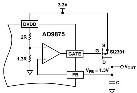
Figure 3b. Connections for a 1.3 V Linear Regulator
