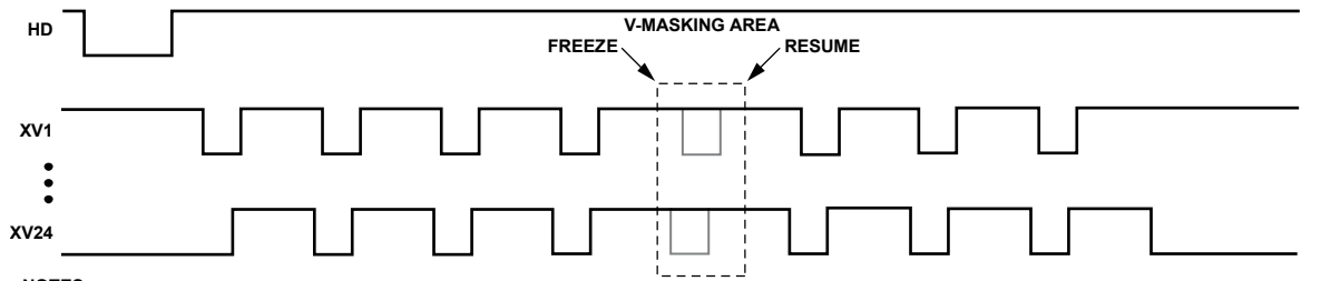
Figure 45. Using FREEZE/RESUME
