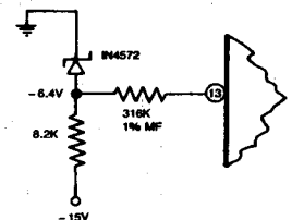
6.4V ZENER REFERENCE REQUIRES -15V SUPPLY
