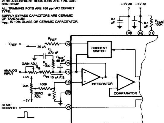
*33 pF FOR ADC-ET86C
