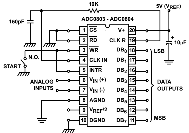
FIGURE 17. FREE-RUNNING CONNECTION
