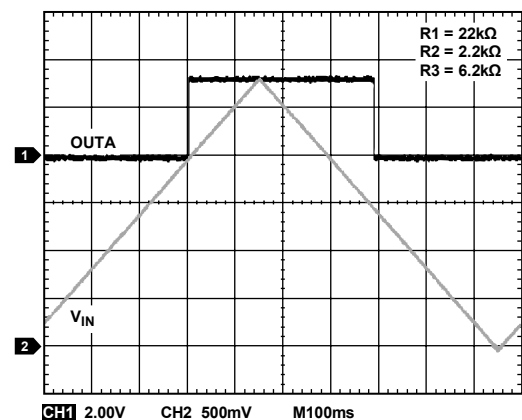
Figure 3. Hysteresis programmed to 513 mV @ V_{IN} on ADCMP341
