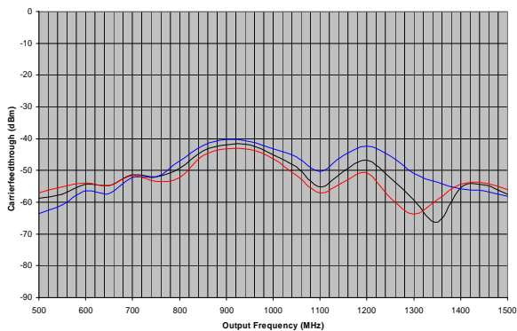
Figure 11. ADL5371 Uncalibrated Carrier Feed through
