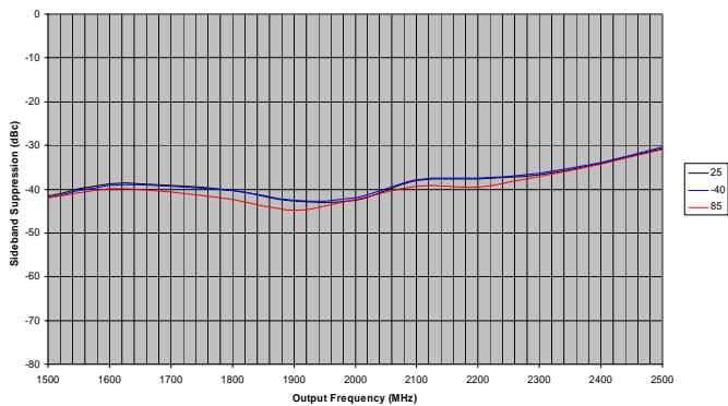
Figure 17. ADL5372 Uncalibrated Undesired Side band
