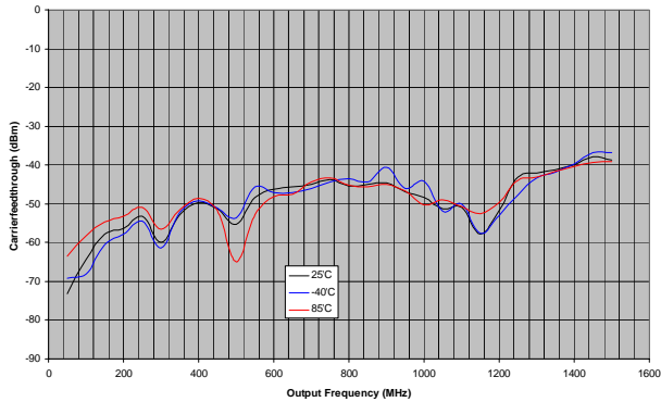
Figure 9. ADL5370 Uncalibrated Carrier Feed through
