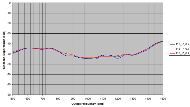
Figure 15. ADL5371 Uncalibrated Undesired Side band
