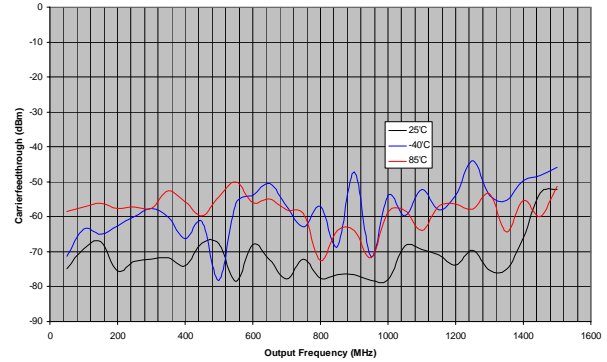
Figure 12. ADL5370 Carrier Feed through with Nulling at 25C
