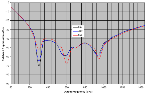
Figure 10. ADL5370 Uncalibrated Undesired Side band
