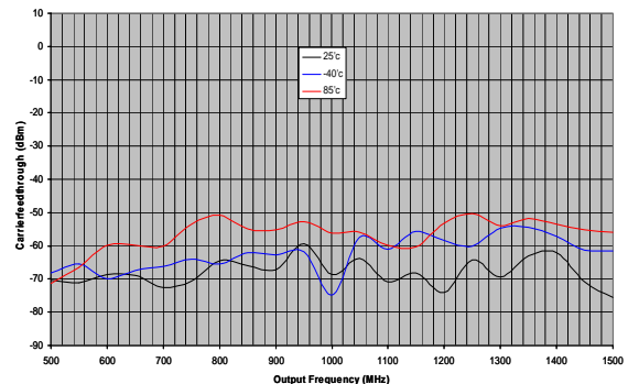
Figure 14. ADL5371 Carrier Feed through with Nulling at 25C
