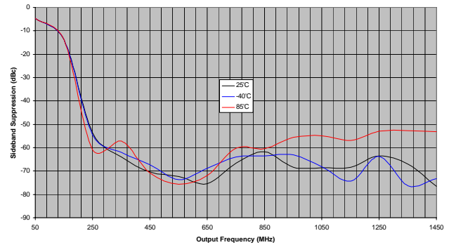
Figure 13. ADL5370 Undesired Sideband with Nulling at 25C
