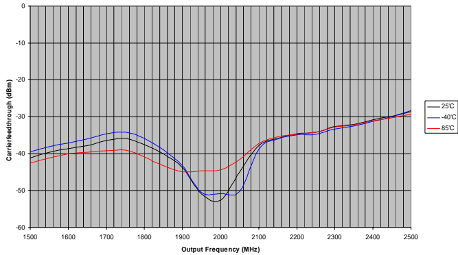
Figure 16. ADL5372 Uncalibrated Carrier Feed through
