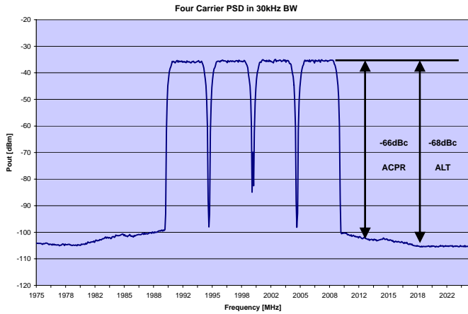
Figure 3. ADL5372 Four Carrier WCDMA Spectrum (Test Model 1-64) @ 2 GHz, Pout = -14.5 dBm per Carrier, ACPR = -66 dBc, Zero IF
