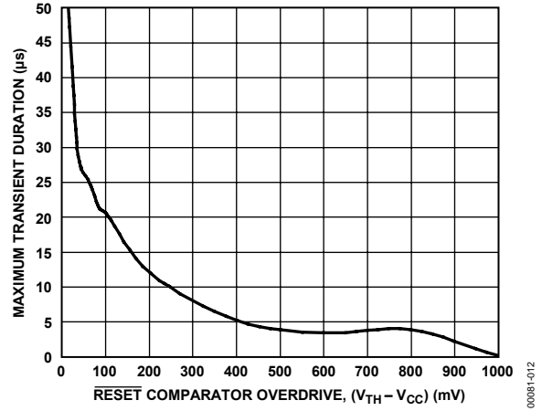
Figure 7. Maximum Transient Duration vs. \overline{\text{RESET}} Comparator Overdrive
