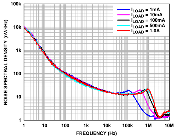
Figure 45. Output Noise Spectral Density, V_{OUT} = 3\text{ V}
