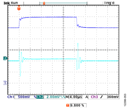
Figure 53. Line Transient Response, 2.5 V to 3 V, I_{LOAD} = 1 A, Adjustable Version, V_{OUT} = 1.2 V, CH1 = V_{IN} , CH2 = V_{OUT}
