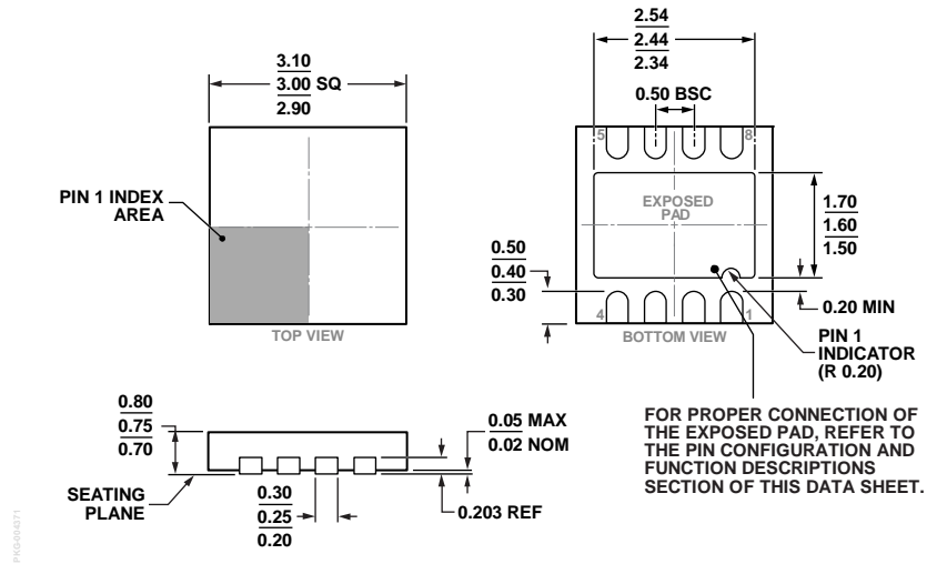
Figure 70. 8-Lead Lead Frame Chip Scale Package [LFCSP_WD] 3 mm × 3 mm Body, Very Very Thin, Dual Lead (CP-8-21) Dimensions shown in millimeters
