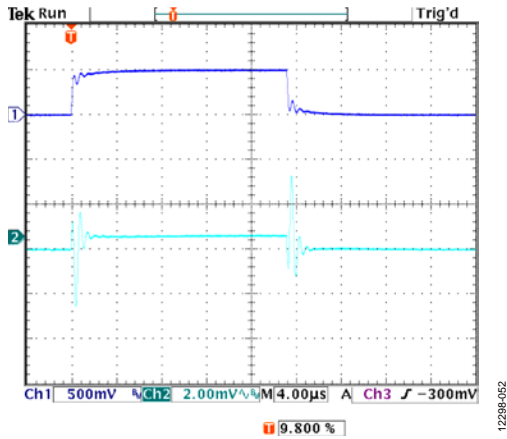
Figure 52. Line Transient Response, 6 V to 6.5 V, I_{LOAD} = 1 A, V_{OUT} = 5 V, CH1 = V_{IN} , CH2 = V_{OUT}
