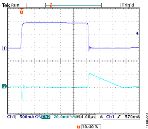
Figure 56. Output Transient Response, V_{OUT} = 5\text{ V} , C_{OUT} = 4.7\ \mu\text{F}
