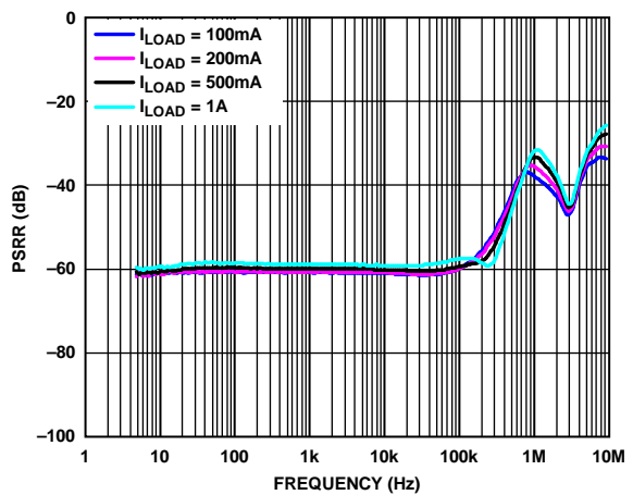
Figure 33. Power Supply Rejection Ratio (PSRR) vs. Frequency, 400 mV Headroom, V_{OUT} = 3 V
