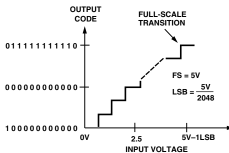
Figure 5. Transfer Function
