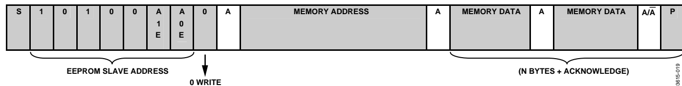
Figure 19. EEPROM Write
