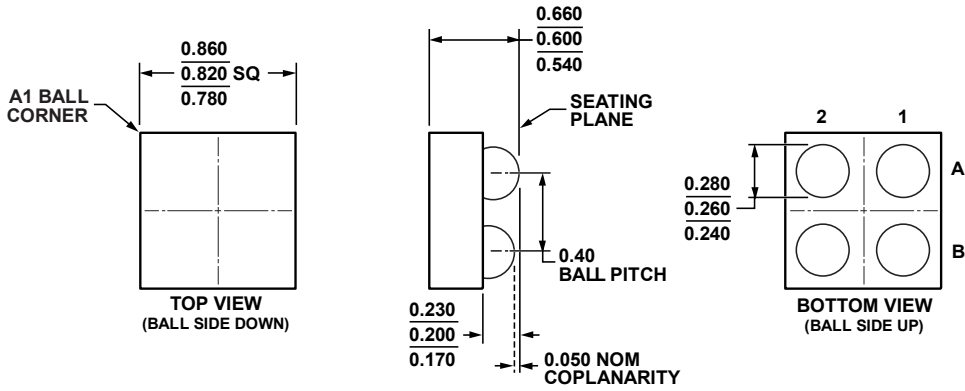
Figure 51. 4-Ball Wafer Level Chip Scale Package [WLCSF] (CB-4-2) Dimensions show in millimeters
