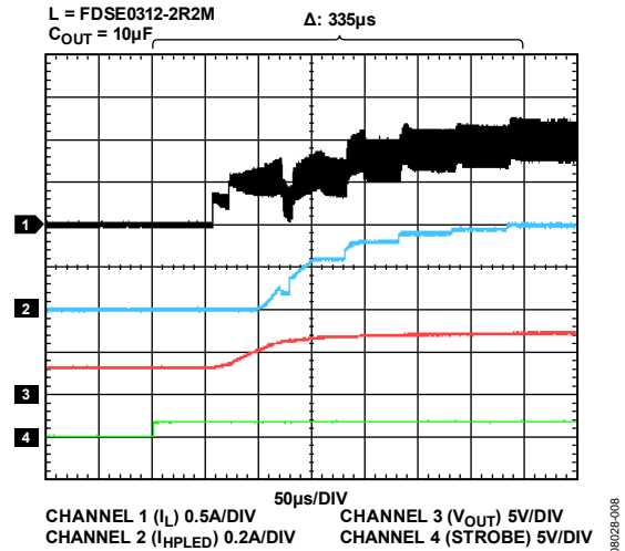
Figure 8. Startup, Two LEDs Flash Mode, I_{LED} = 400\text{ mA} , V_{IN} = 3.6\text{ V}
