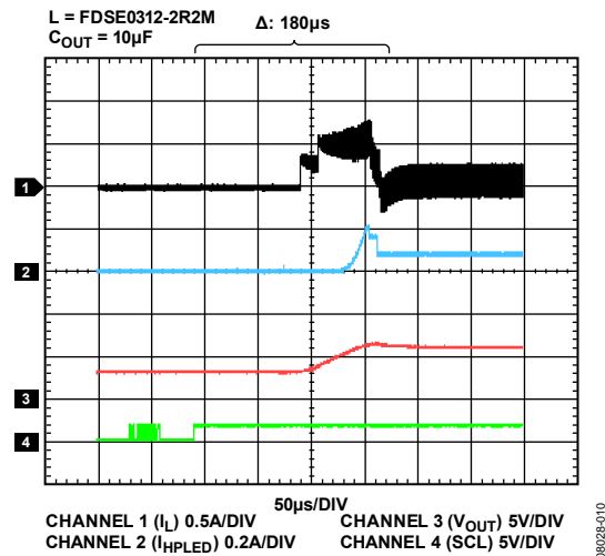
Figure 10. Startup, Two LEDs Torch Mode, I_{LED} = 40\text{ mA} , V_{IN} = 3.6\text{ V}
