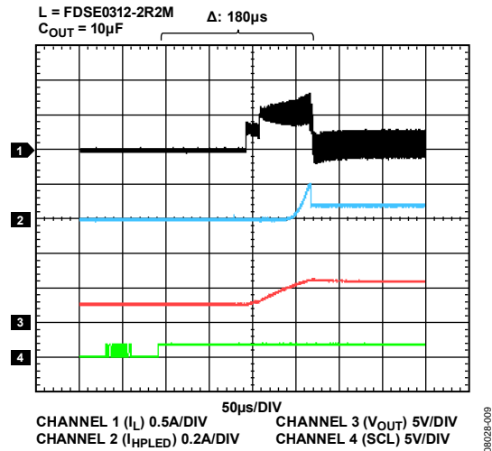
Figure 9. Startup, Two LEDs Assist Light Mode, I_{LED} = 40\text{ mA} , V_{IN} = 3.2\text{ V}
