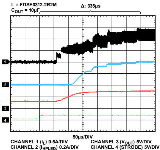
Figure 7. Startup, Two LEDs Flash Mode, I_{LED} = 400\text{ mA} , V_{IN} = 3.2\text{ V}
