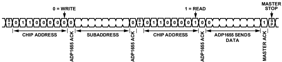
Figure 32. I 2 C Single Register Read Sequence
