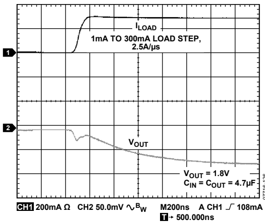
Figure 28. Output Transient Response, C_{OUT} = 4.7 \mu\text{F}
