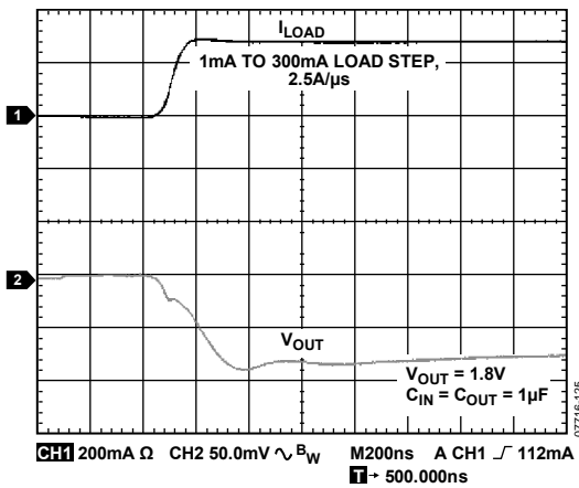
Figure 27. Output Transient Response, C_{OUT} = 1 \mu\text{F}
