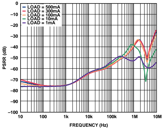
Figure 35. Power Supply Rejection Ratio vs. Frequency, V_{OUT} = 3.3\text{ V} , V_{IN} = 4.8\text{ V}
