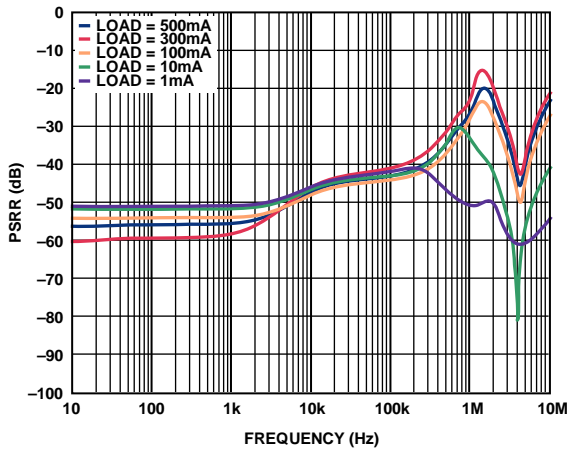
Figure 37. Power Supply Rejection Ratio vs. Frequency, V_{OUT} = 3.3\text{ V} , V_{IN} = 3.8\text{ V}
