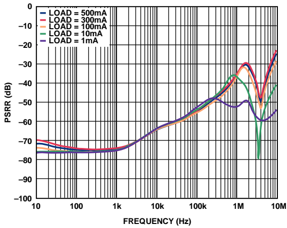
Figure 36. Power Supply Rejection Ratio vs. Frequency, V_{OUT} = 3.3\text{ V} , V_{IN} = 4.3\text{ V}
