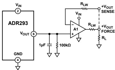
Figure 23. Advantage of Kelvin Connection
