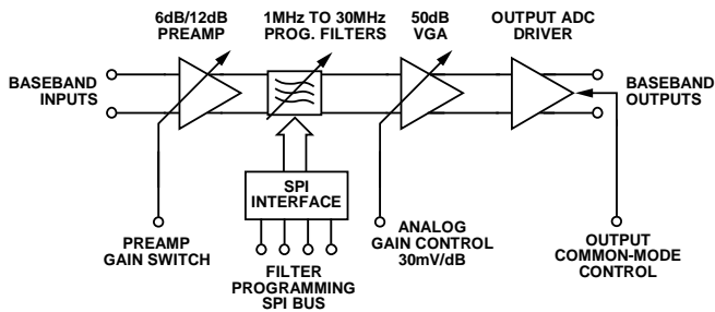
Figure 41. Signal Path Block Diagram for a Single Channel of the ADRF6510
