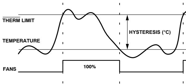
Figure 28. \overline{\text{THERM}} Limit Operation
