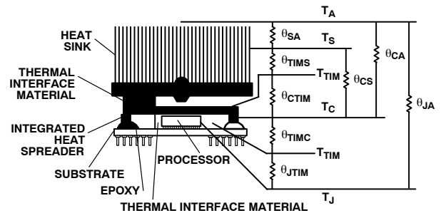
Figure 65. Thermal Model
