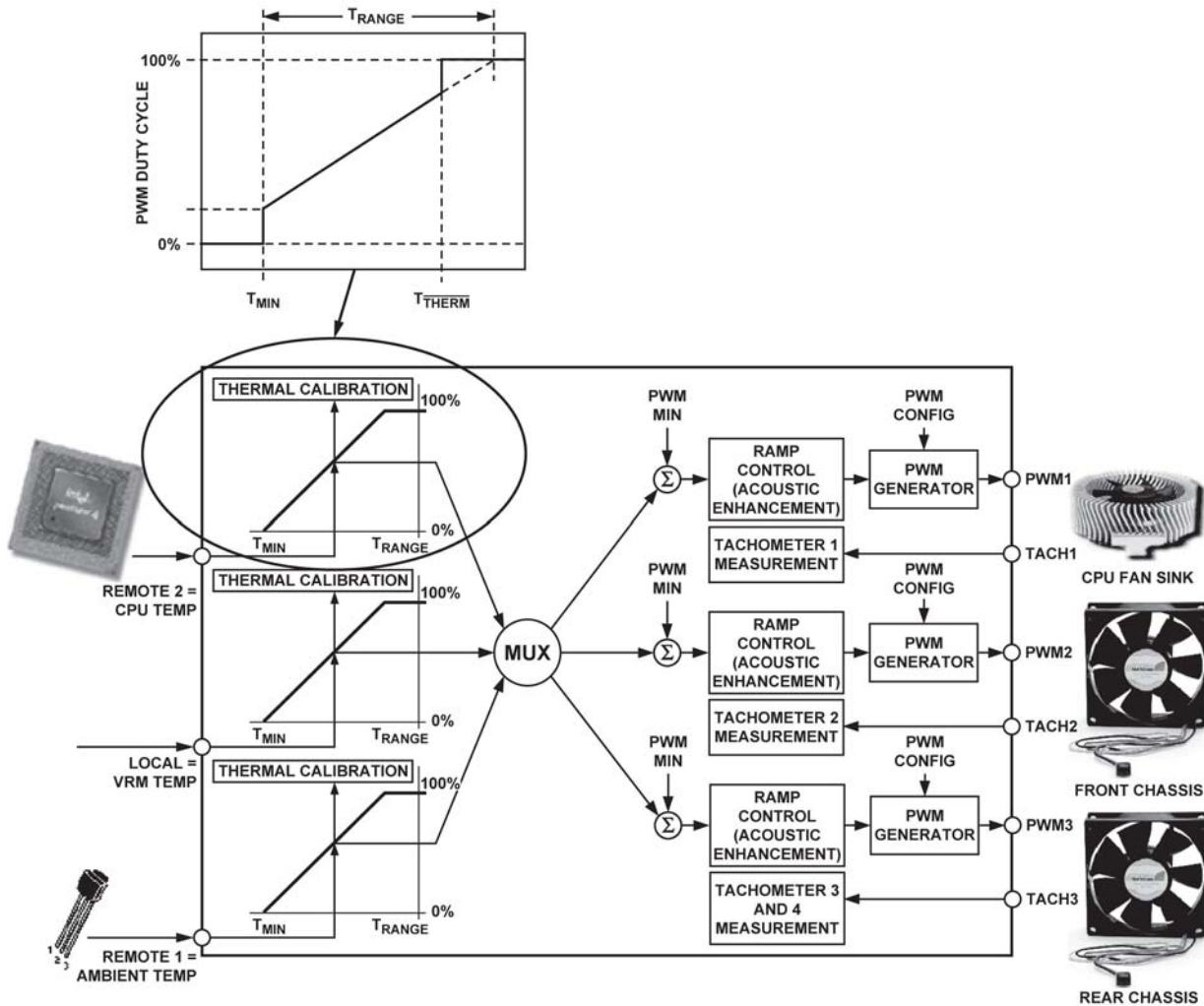
Figure 62. How \overline{THERM} Relates to Automatic Fan Control
