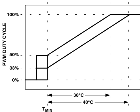
Figure 57. Adjusting PWM MIN Affects T RANGE
