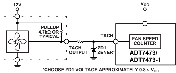
Figure 42. Fan with Strong TACH Pullup to > V CC or Totem-Pole Output, Clamped with Zener and Resistor
