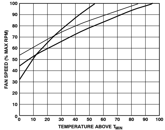
Figure 61. T_{RANGE} and % Fan Speed Slopes for VRM, Ambient, and CPU Temperature Channels
