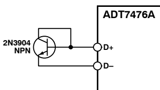
Figure 26. Measuring Temperature Using an NPN Transistor
