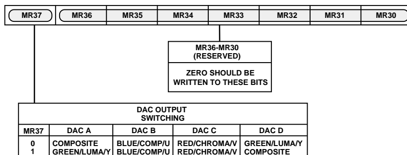
Figure 40. Mode Register 3
