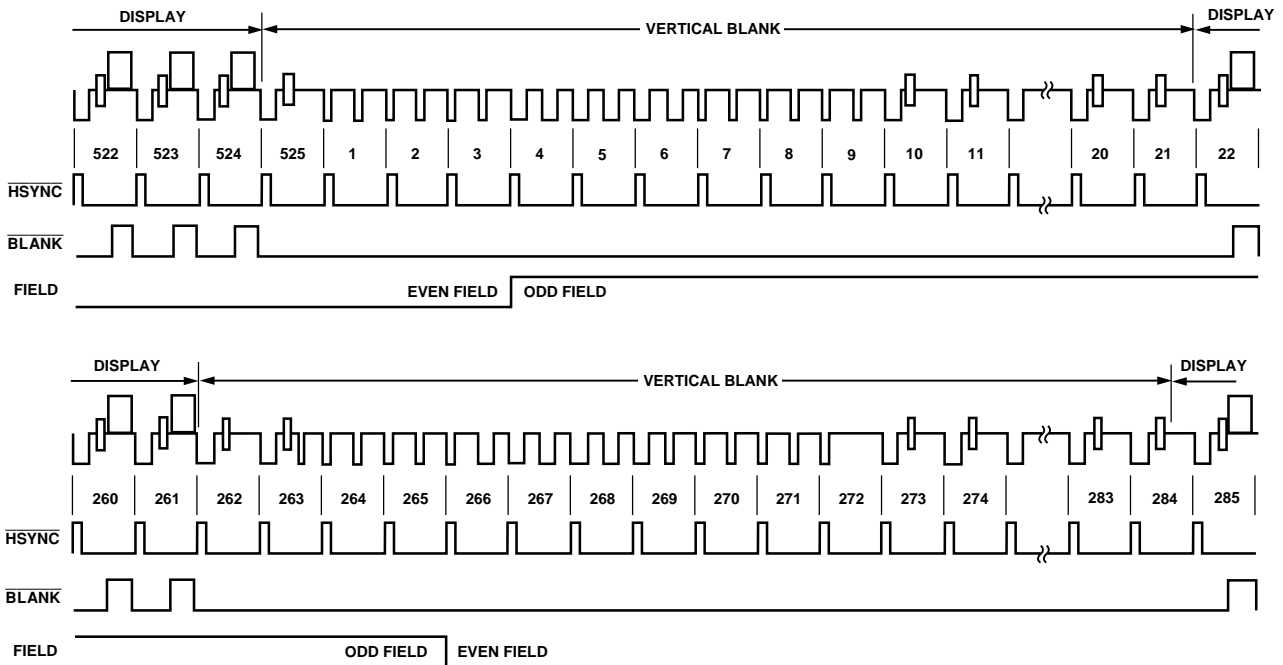
Figure 24. Timing Mode 3 (NTSC)
