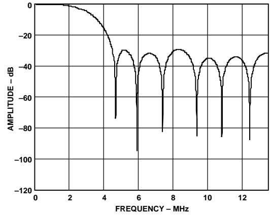
Figure 8. PAL Notch Filter
