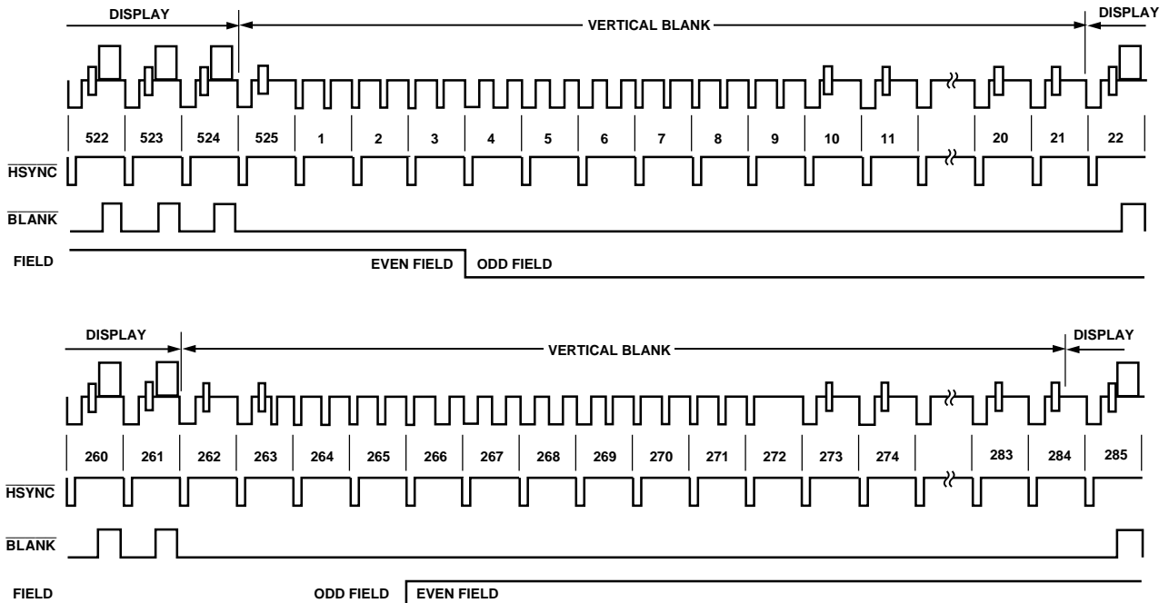
Figure 17. Timing Mode 1 (NTSC)
