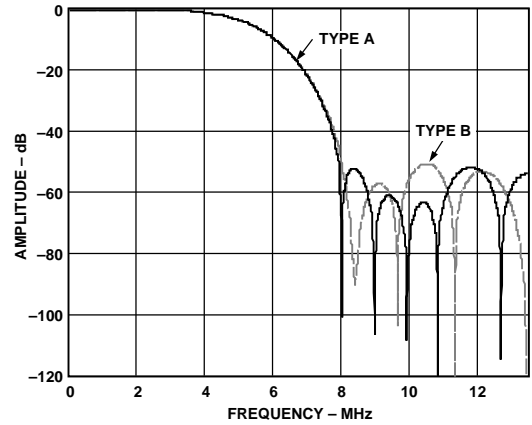
Figure 7. PAL Low-Pass Filter
