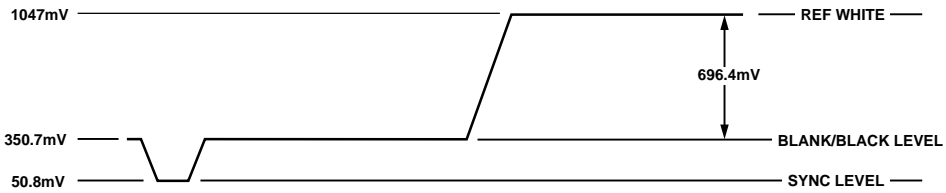
Figure 53. PAL Luma Video Levels
