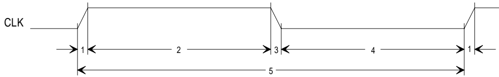
Figure 6: CLK Characteristics
