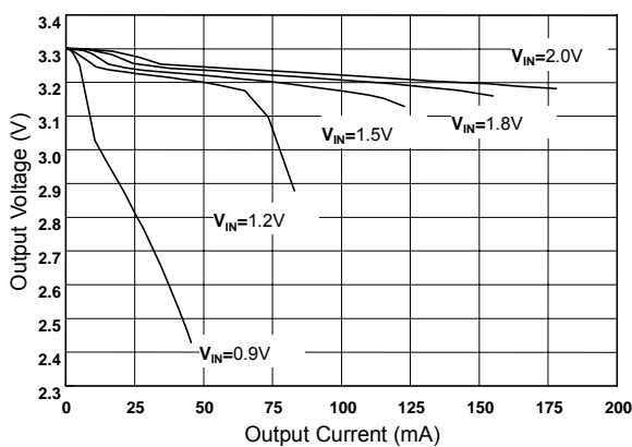
AIC1638-33 Load Regulation (L=100μH, CD54)
