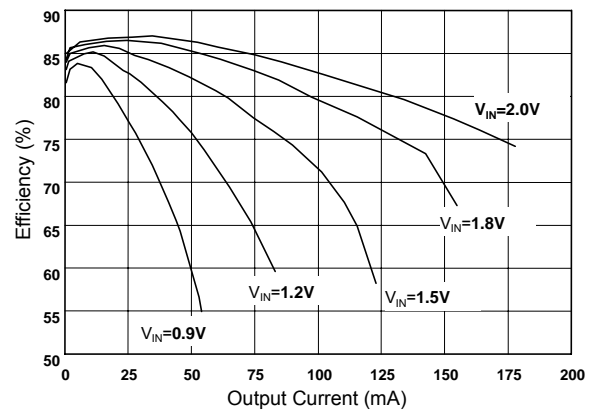
AIC1638-33 Efficiency (L=100μH, CD54)
