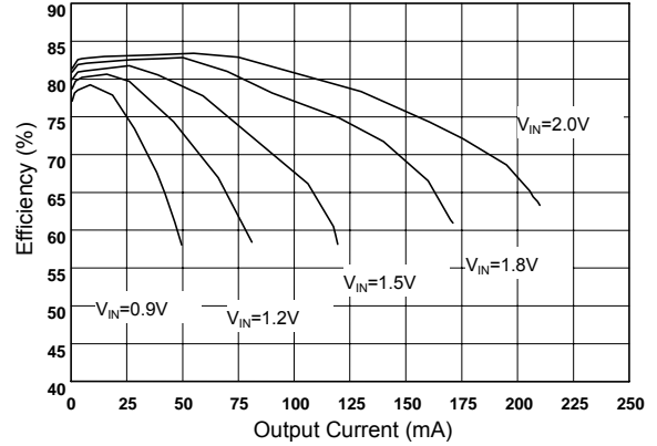
AIC1638-33 Efficiency (L=47 \mu H, CD54)
