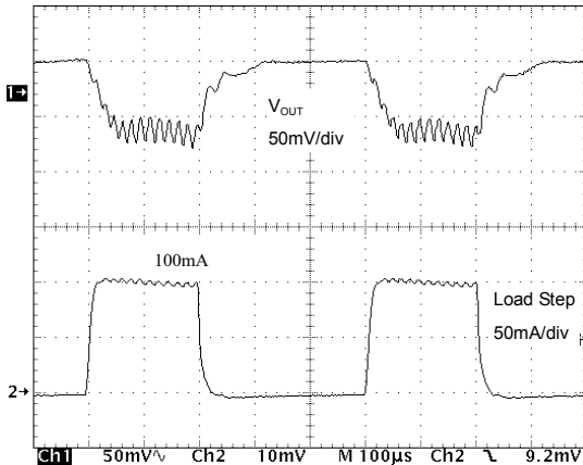
Load Transient Response (L=100µH, Co=47µF, VIN=2V)
