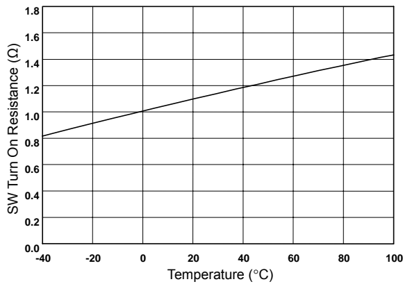
AIC1638-30 SW On Resistance vs Temperature
