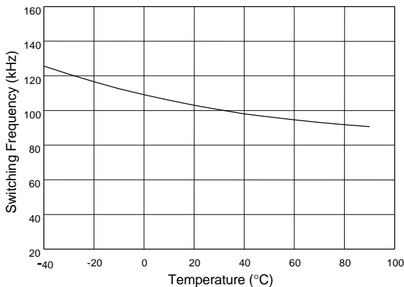
Fig. 5 AIC1642-27 Switching Frequency vs. Temperature
