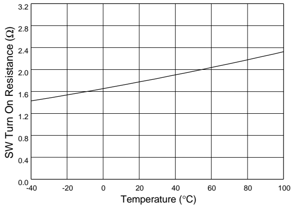
Fig. 31 AIC1642-50 SW On Resistance vs. Temperature
