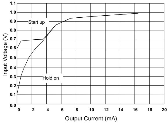
Fig. 19 AIC1642-33 Start-up & Hold-on Voltage (L=100μH)
