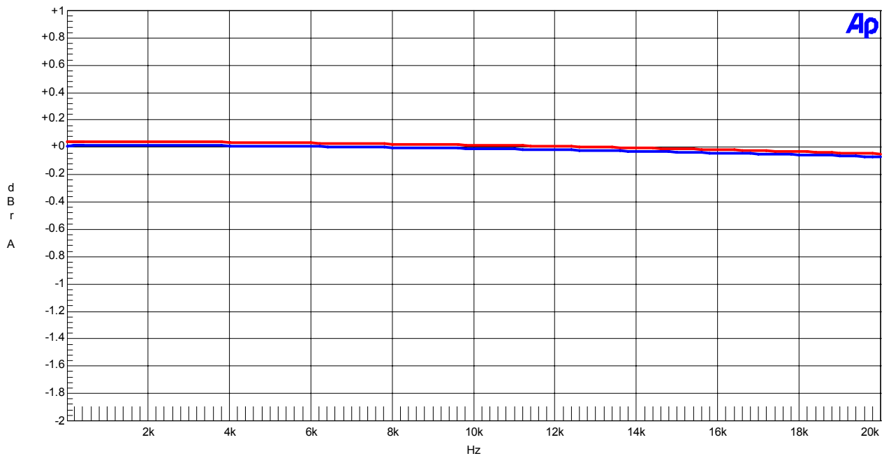
Figure 8 Frequency Response (Input level=0dBFS)
