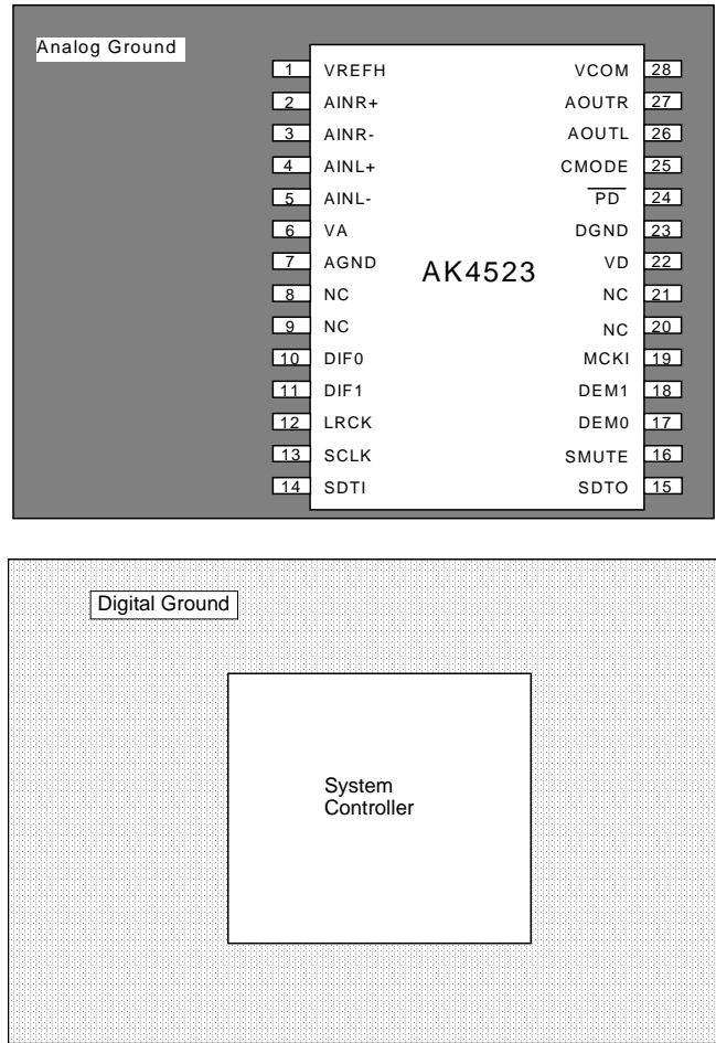
Figure 8. Ground Layout
