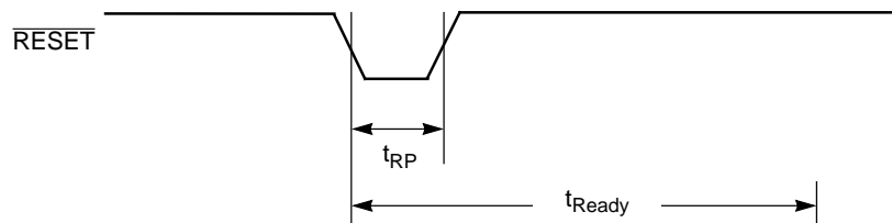
Figure 18. \overline{RESET} Timing Diagram
