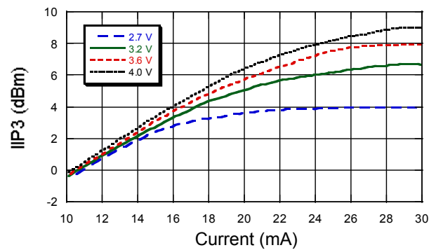
High Gain Mode: IIP3 vs. Current and Voltage
