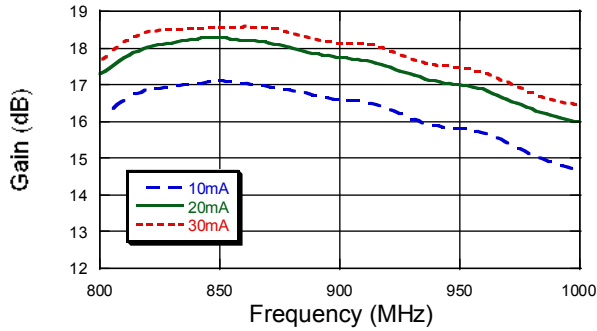
High Gain Mode: Gain vs. Current
