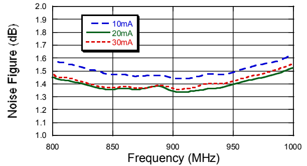
High Gain Mode: Noise Figure vs. Current
