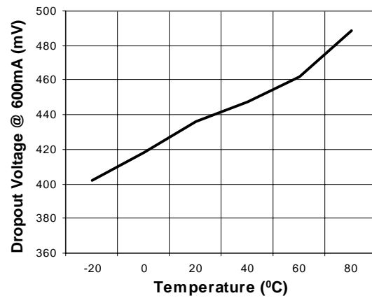
Dropout Voltage vs. Temp.
