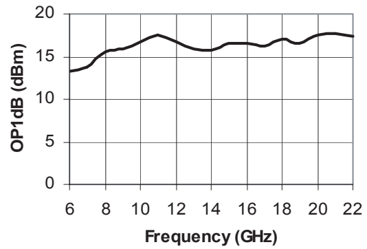
Figure 4a. Output P-1dB
