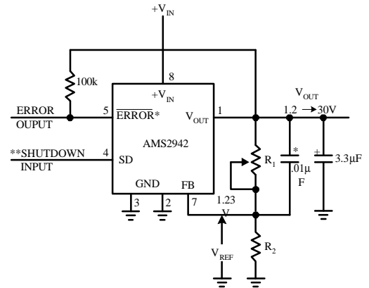
FIGURE 2. Adjustable Regulator
