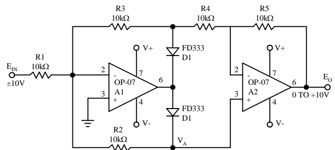
Precision Absolute Value Circuit
