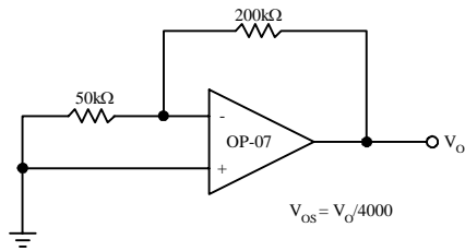
TYPICAL OFFSET VOLTAGE TEST CIRCUIT
