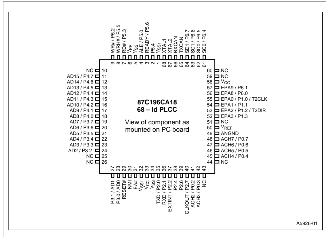
Figure 3. 87C196CA 68-Pin PLCC Package Diagram
