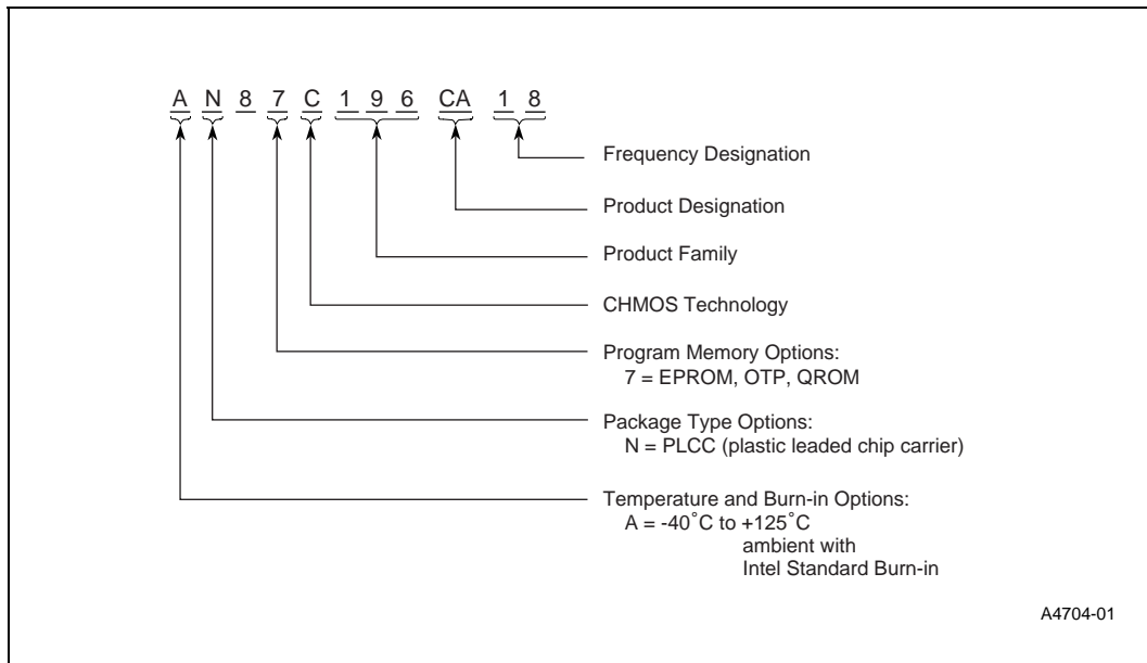
Figure 2. 87C196CA Nomenclature
