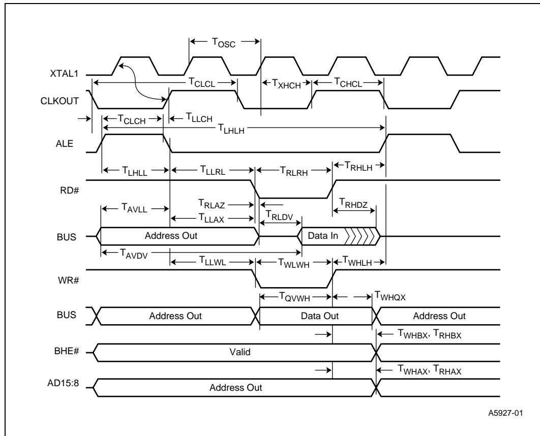
Figure 5. System Bus Timing
