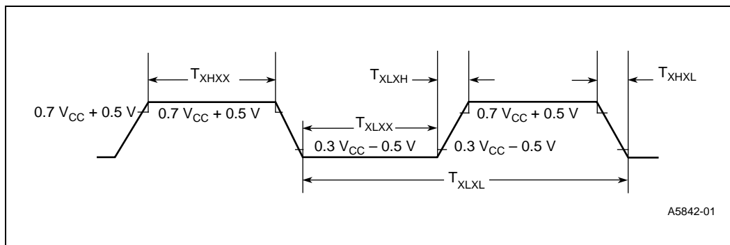
Figure 7. External Clock Drive Waveforms
