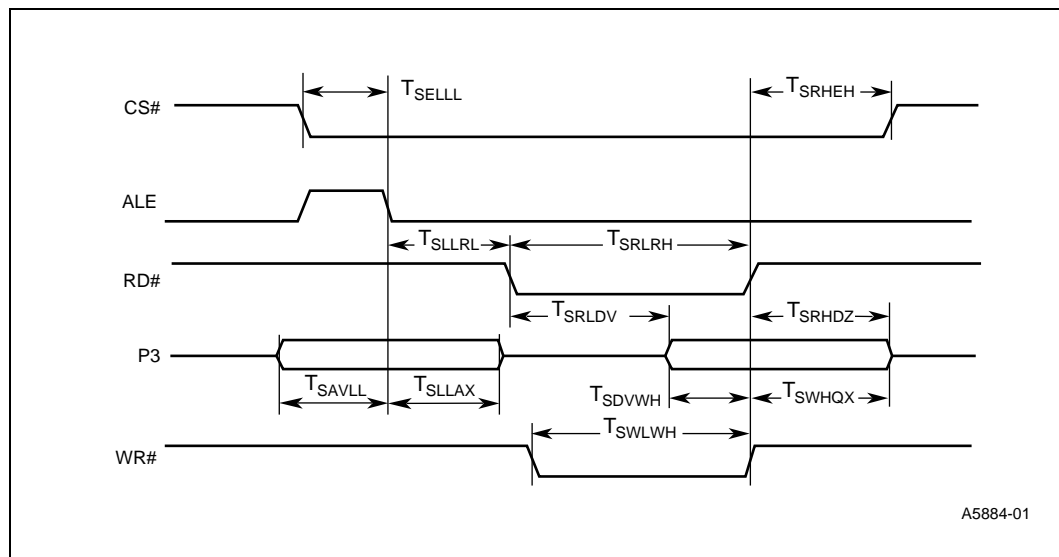
Figure 14. Slave Port Waveform (SLPL = 1)
