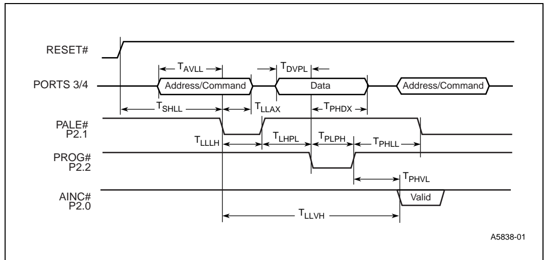
Figure 11. Slave Programming Mode in Word Dump or Data Verify Mode with Auto Increment
