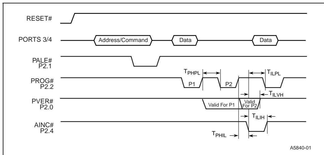
Figure 12. Slave Programming Mode Timing in Data Program Mode with Repeated PROG Pulse and Auto Increment
