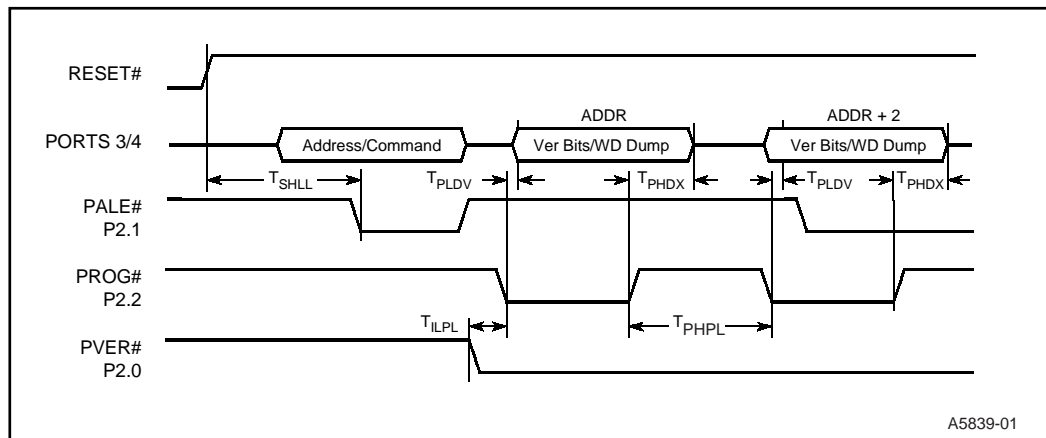
Figure 11. Slave Programming Mode in Word Dump or Data Verify Mode with Auto Increment
