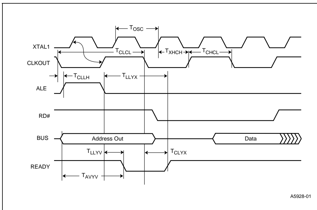
Figure 6. READY Timing
