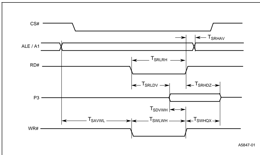
Figure 13. Slave Port Waveform (SLPL = 0)
