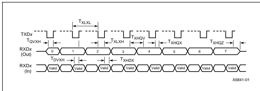
Figure 15. Serial Port Waveform—Shift Register Mode
