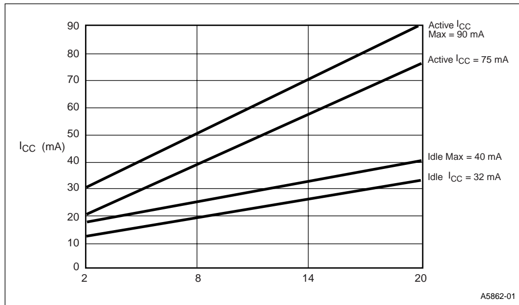
Figure 4. 87C196CA I CC vs. Frequency
