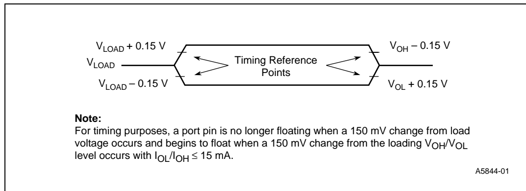
Figure 9. Float Waveforms
