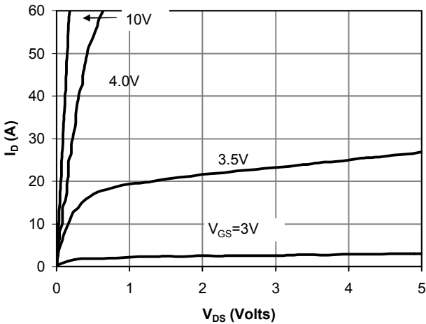
Fig 1: On-Region Characteristics
