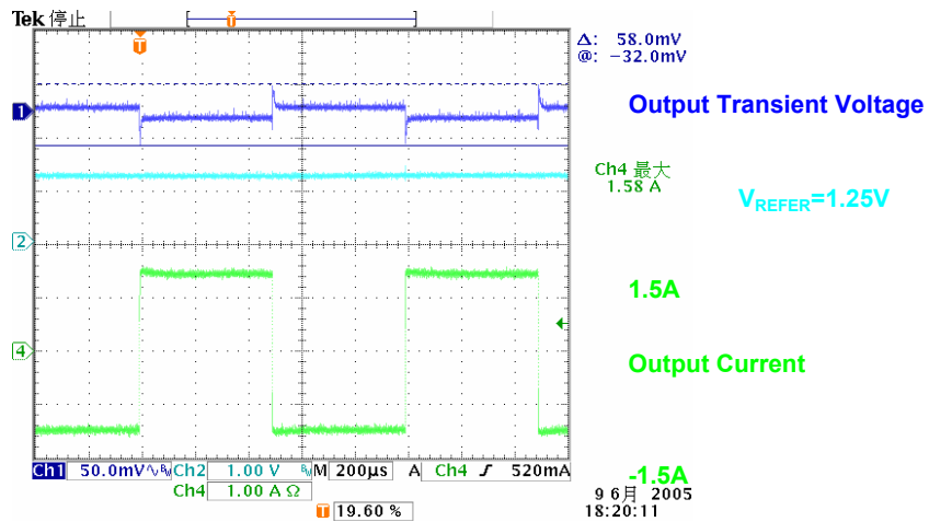
V_{IN}=2.5V , V_{CNLT}=3.3V , V_{REFER}=1.25V , Temp(IC\ Body) = 98^{\circ}C Fig 7. Transient Response
