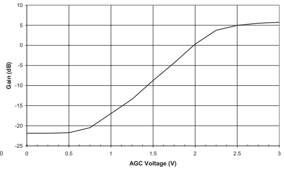
Figure 10: Gain vs. AGC Voltage ( T_A = +25\text{ }^\circ\text{C} , V_{CC} = +5\text{ V} )
