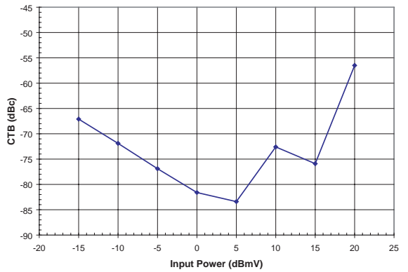
Figure 9: CTB vs. Input Power (T C = +25 °C, V CC = +5 V, f = 439 MHz, P OUT = +6 dBmV, 135 channel flat input)
