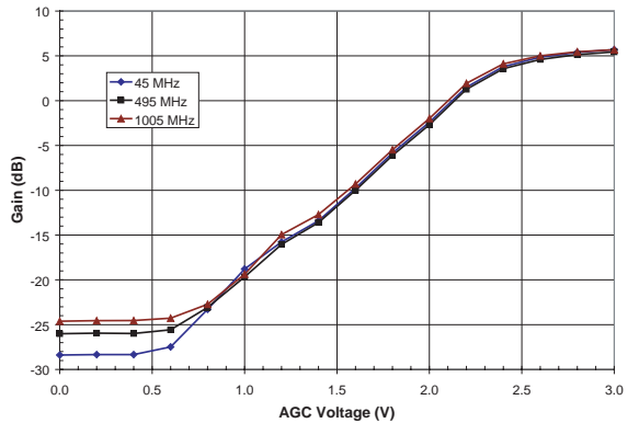
Figure 11: Gain vs. AGC Voltage (T C = +25 °C, V CC = +5 V)
