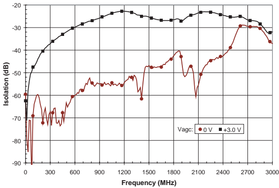
Figure 10: Output Port-to-Port Isolation vs. Frequency (T C = +25 °C, V CC = +5 V)
