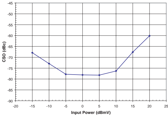
Figure 8: CSO vs. Input Power (T C = +25 °C, V CC = +5 V, f = 77 MHz, P OUT = +6 dBmV, 135 channel flat input)
