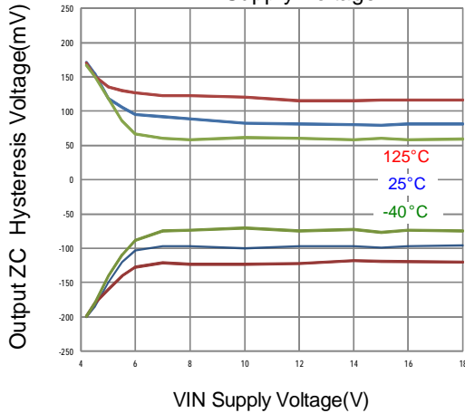
Output ZC Hysteresis Voltage vs. VIN Supply Voltage
