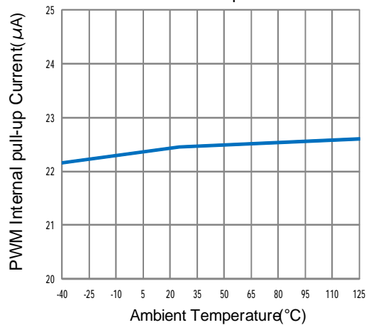
PWM Internal pull-up Current vs. Ambient Temperature
