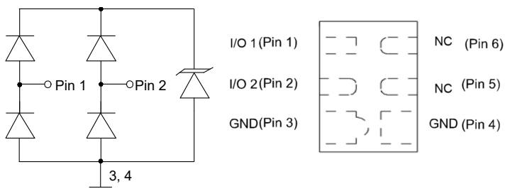
Circuit Schematic
