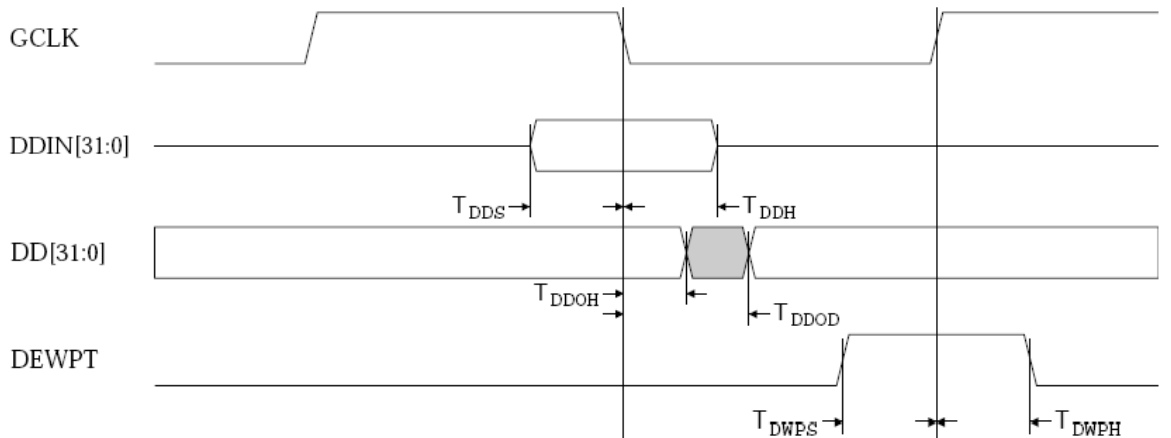
Figure 8-7 ARM9TDMI data data bus timing
