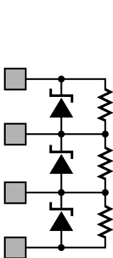
Figure 14. Simple Trim Setup with 8 Trim Steps.
