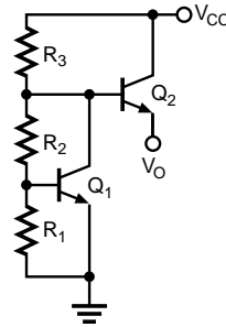
Figure 9. V_{BE} Multiplied Regulator. V_{OUT} = V_{BE} * R_2 / R_1
