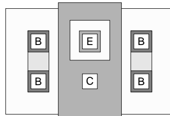
Vertical PNP
