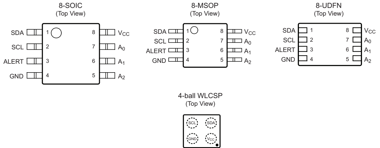
Figure 1. Pin Configurations
