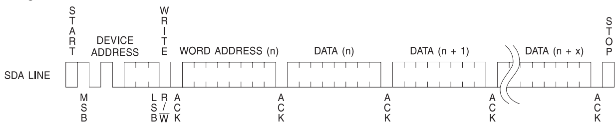
Figure 4. Page Write
