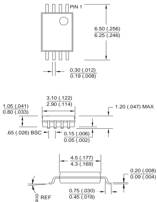
8T , 8-Lead, 0.170" Wide, Thin Shrink Small Outline Package (TSSOP) Dimensions in Millimeters and (Inches)
