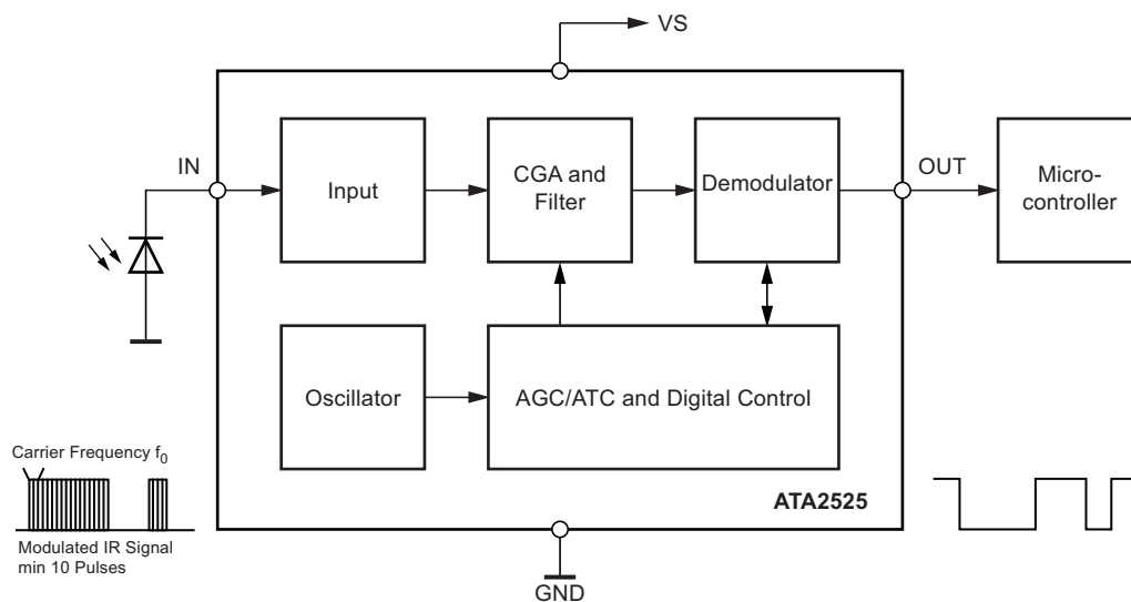
Figure 1-1. Block Diagram
