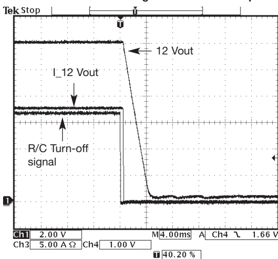
Figure 11: Remote Control Turning-off Characteristic. Vin = 48 Volts, Turning-off into Full Load for 12 Vout and 3.3 Vout
