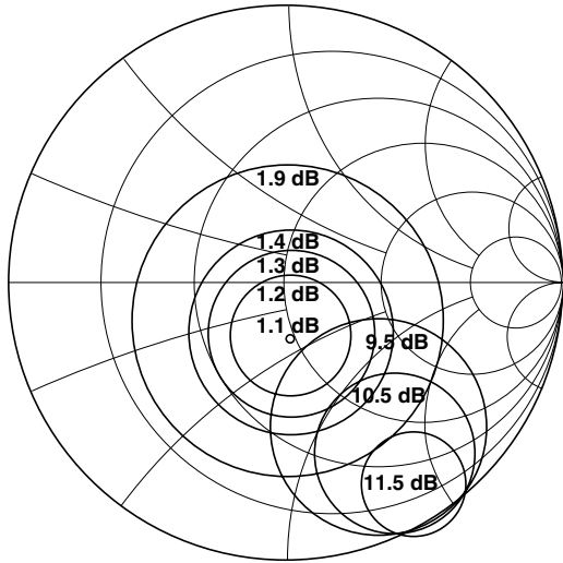
Figure 9. Smith Chart with Noise Figure and Available Gain Circles at 12 GHz, V_{DS} = 1.5\text{ V} , I_D = 10\text{ mA} .
