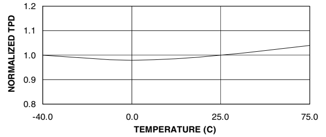
NORMALIZED T_{PD} VS. TEMP
