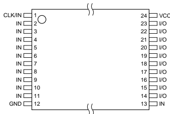
DIP/SOIC
